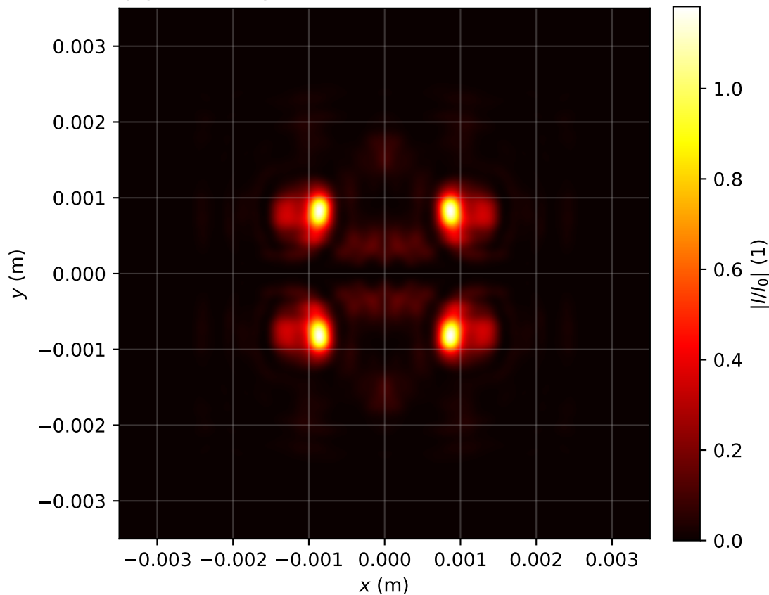
Intensity profile I(x, y, z = 2.388)/I_0 , P_{in}=9.0P_{cr} , artificial time
